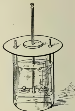
From A. S. T. M. Standards. FIG. 177.—B. and R. Fusing-Point Tester.
